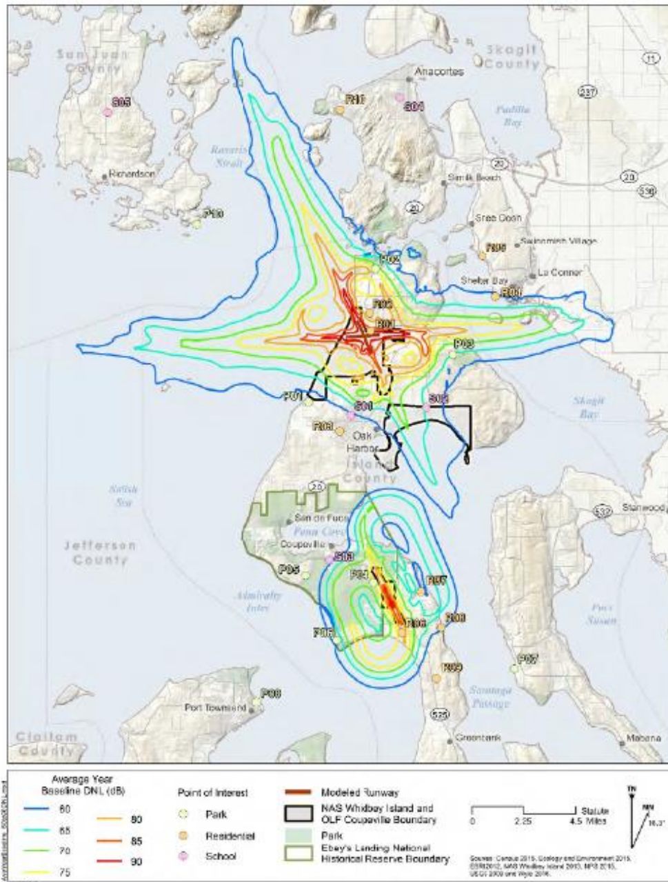
Figure 4-2. DNL Contours for AAD Aircraft Events for the Average Year Baseline Scenario
